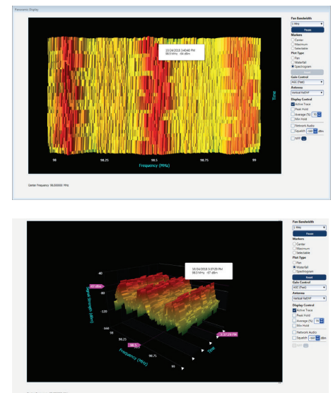
› Fig. 12 – 3D Waterfall, Spectrogram Windows
