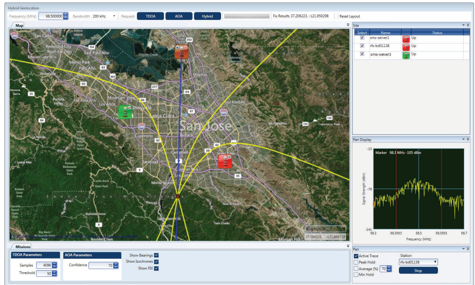
› Figure 6 - TCI Scorpio Hybrid Geolocation
