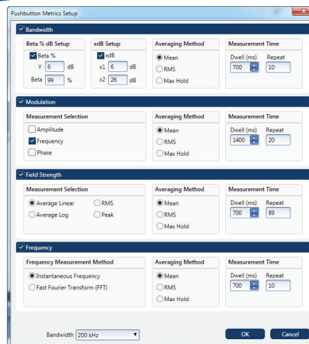
Figure 5 – Pushbutton DF/Metrics Window, Metrics Setup Pop-up Window
