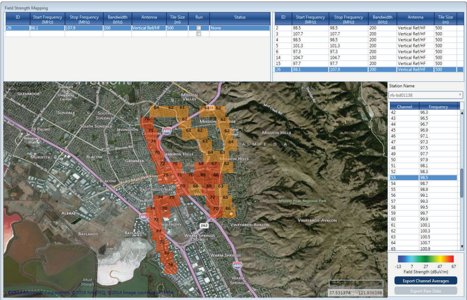
➤ Figure 19 – Field Strength Mapping Window
