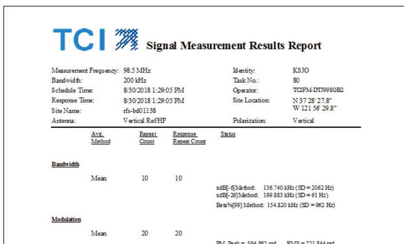
› Figure 21 – Example Scheduled (Calendared) Task Results Report
