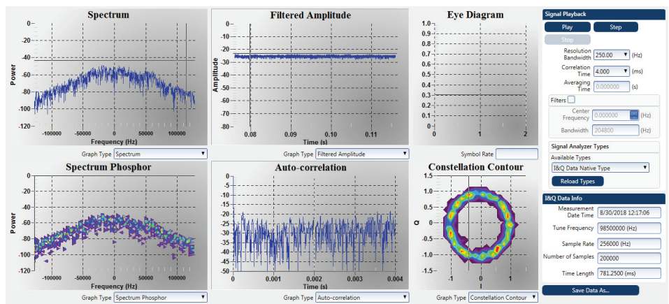
› Figure 23 – Digital Signal Analysis Feature
