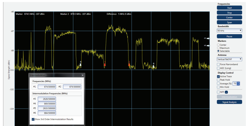
› Figure 22 – TCI Spectrum Analyzer
