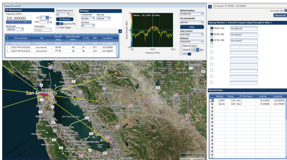
Figure 10 – Netted DF screen, showing FIX for two-site bearing measurement
