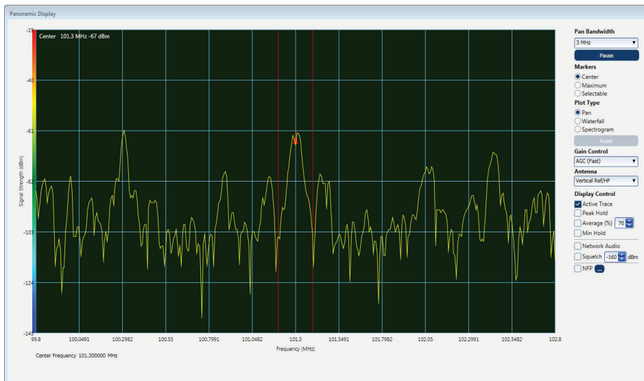
› Figure 11 – Panoramic (or Pan) Display Window
